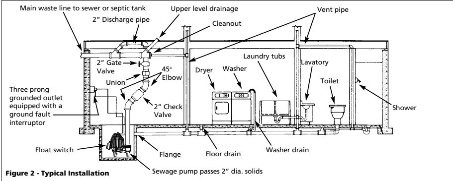
Figure 2 - Typical Installation
